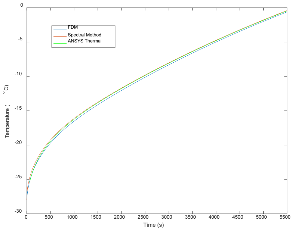
Figure 9: Comparison of corner temperature from three methods FDM, Spectral Method, and ANSYS® Multiphysics thermal simulation
