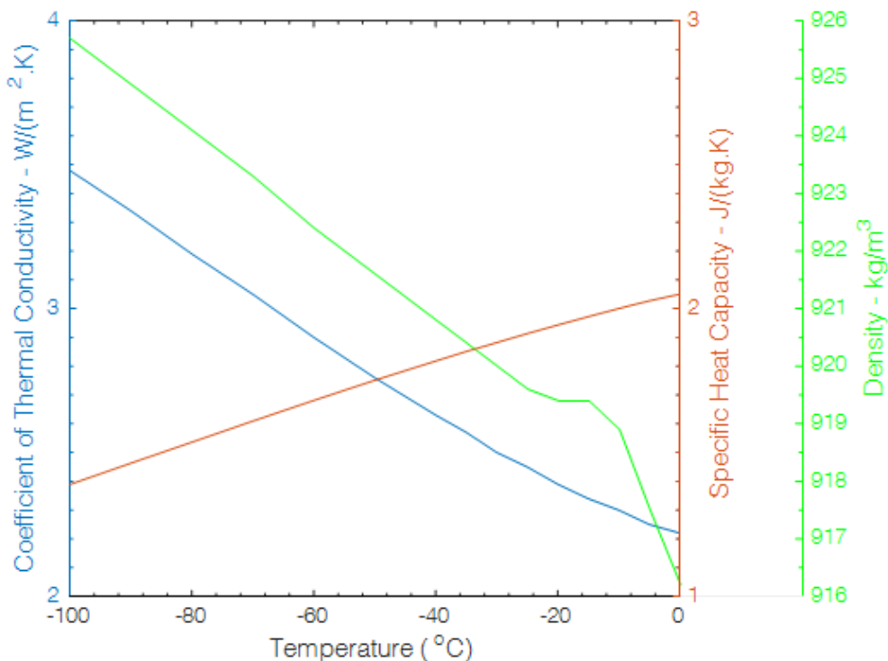
Figure 4: Variation in physical and thermal properties of ice with temperature. [8]
