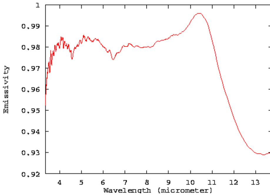
Figure 2: Emissivity of ice with wavelength( \mu\text{m} ) [3]
